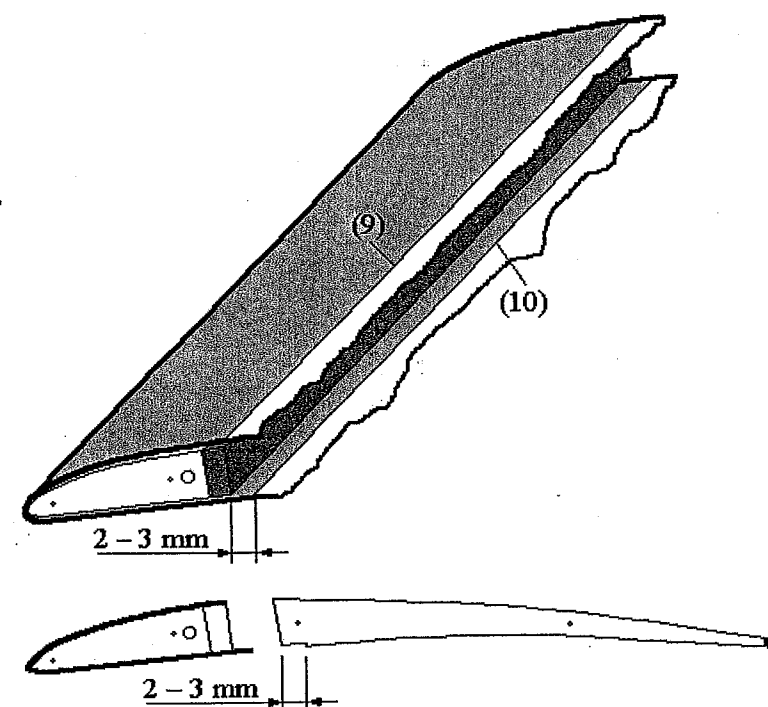
Figure 4. Adjustment of the „shell” on the wing upper and lower side
