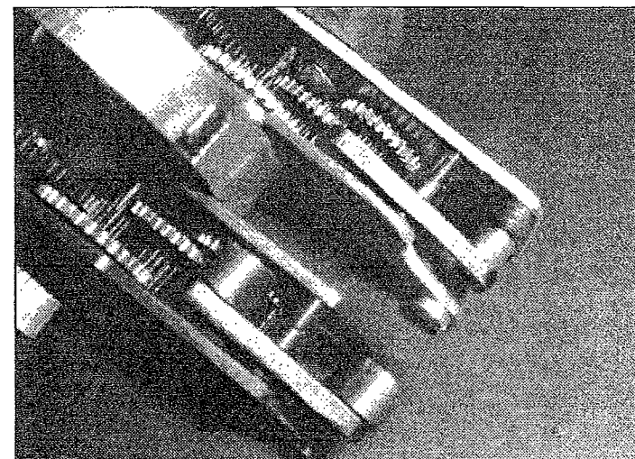
Fig. 2. The clock on the left uses large brass weights to slow the timer. The one on the right has no added weights. This technique works well, within limits. It isn't a precise adjustment, but is effective.
