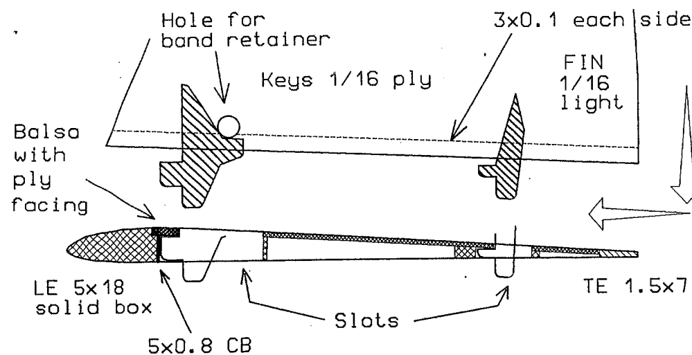
6% HLG AIRFOIL Scarlette (Mean chord 150) (dm 2 )
