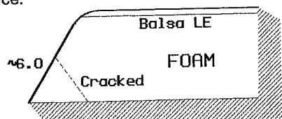
New SALZER wing B.6456-f
