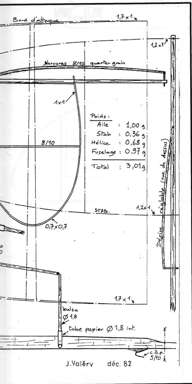
THE "WILFLY" PUSHER MONO
